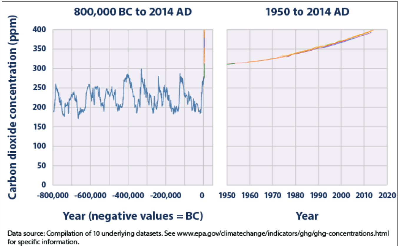
Figure 9-1. Global Carbon Dioxide Concentrations Over Time
