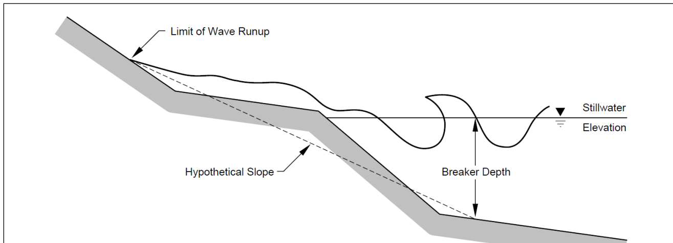
Figure 6-6. Wave Run-Up
